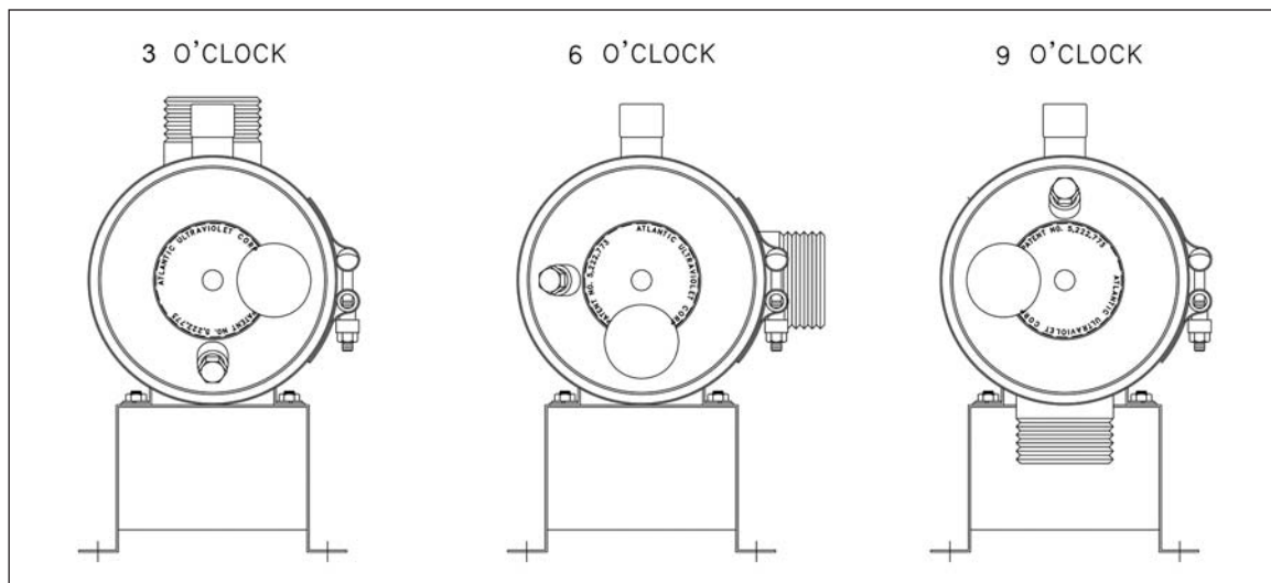
Figure 3 - Recommended Positions of Inlet/Outlet Fittings
