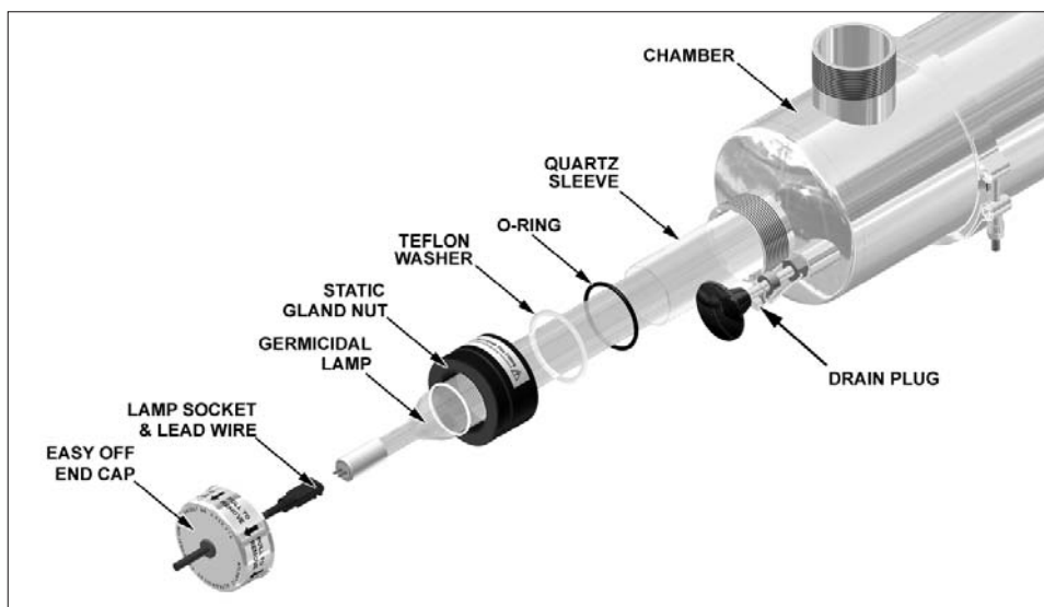
Figure 6 - Quartz Sleeve Cleaning or Replacement
