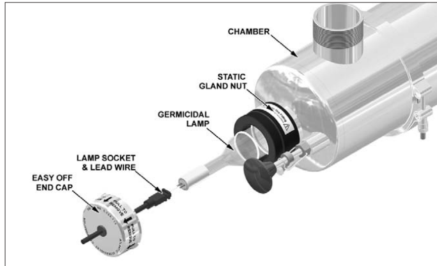
Figure 5 - Lamp Replacement
