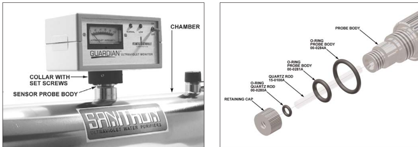
Figure 8 - Ultraviolet Monitor and Sensor Probe
