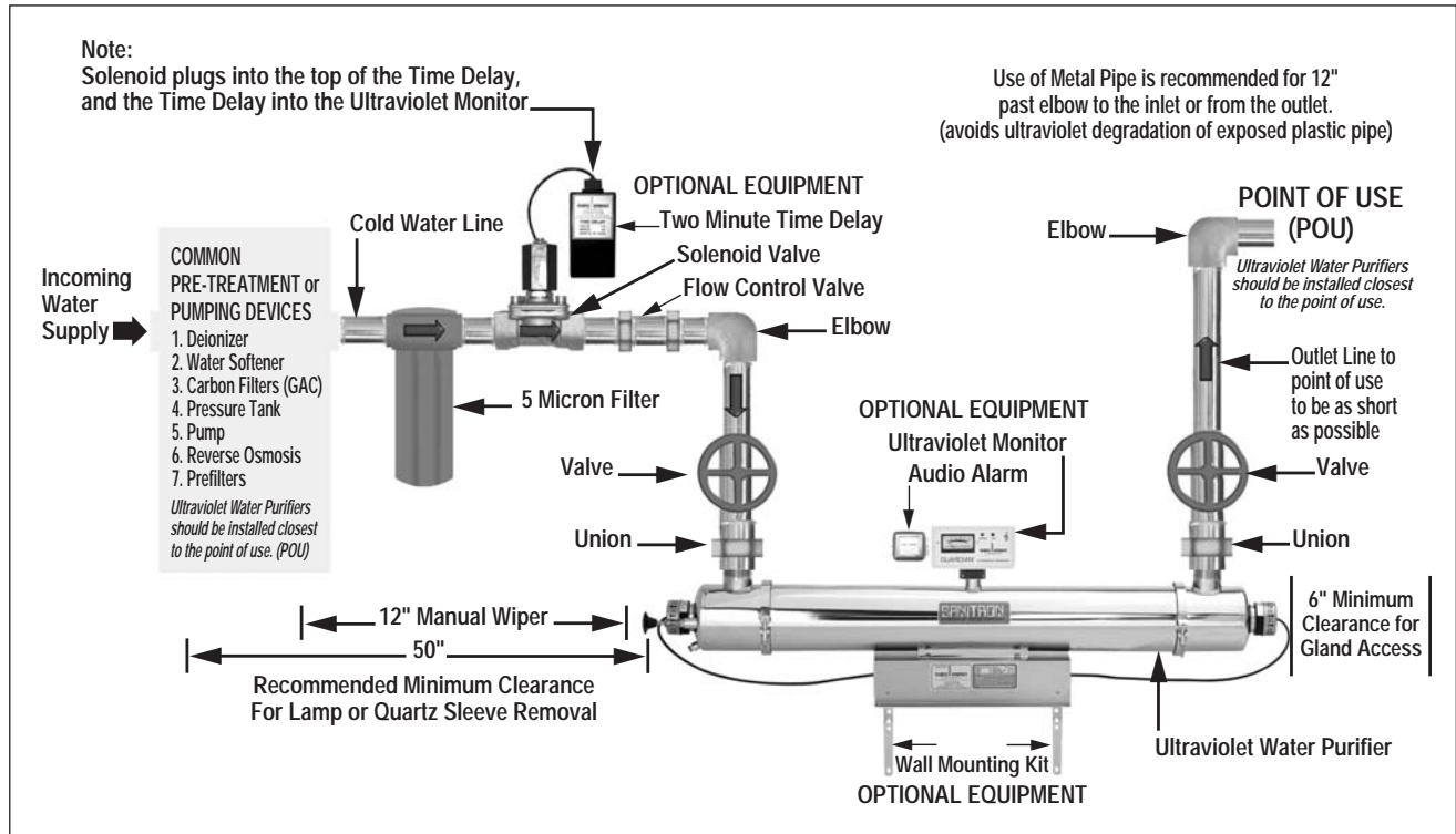
Figure 2 - Recommended Installation
