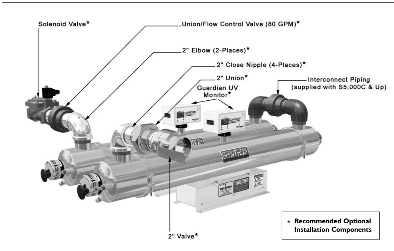
Figure 1 - (1) S5,000C Shown With Recommended Optional Installation Components
