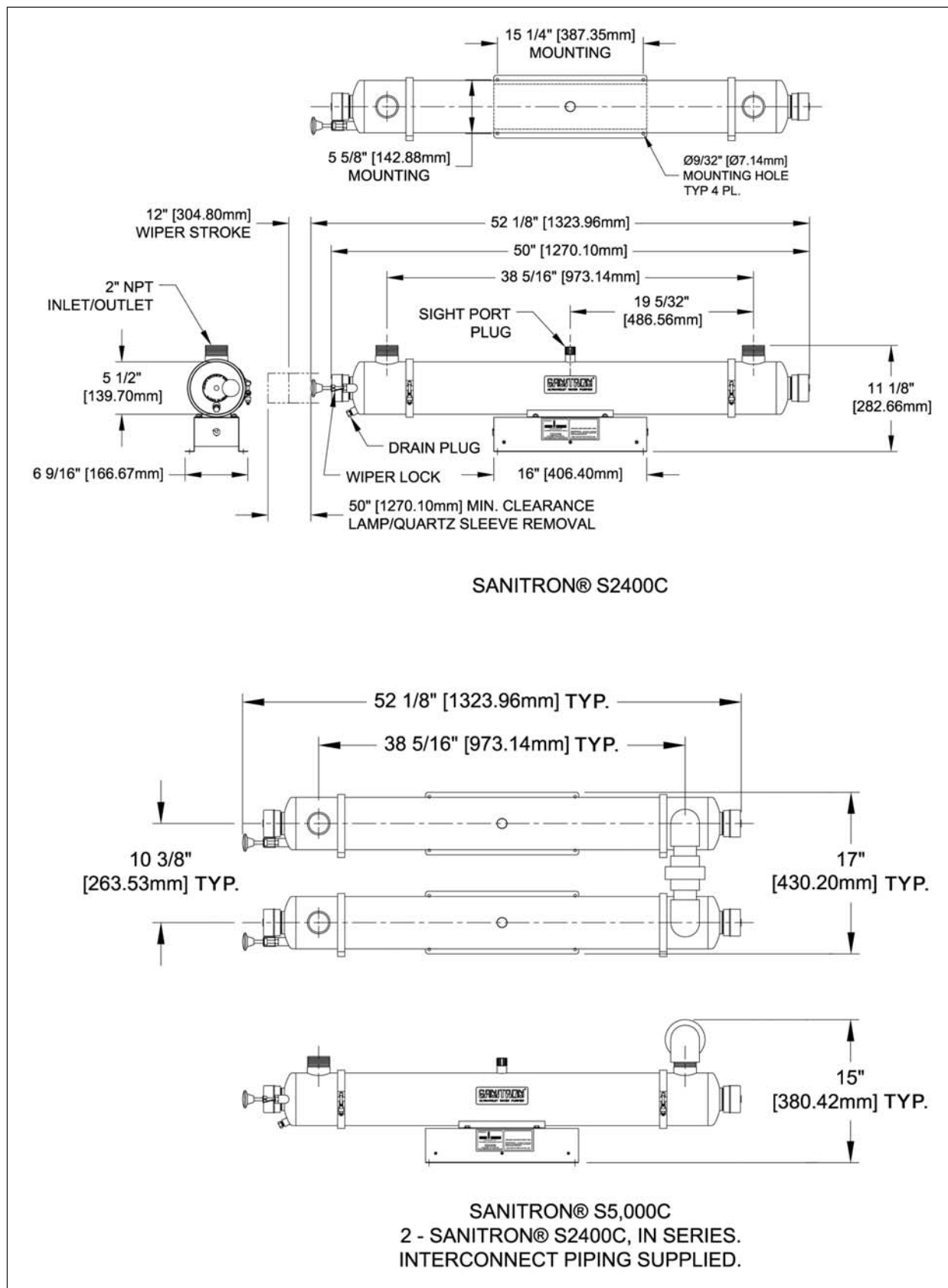
Figure 10 - S2400C & S5,000C Dimensional Data
