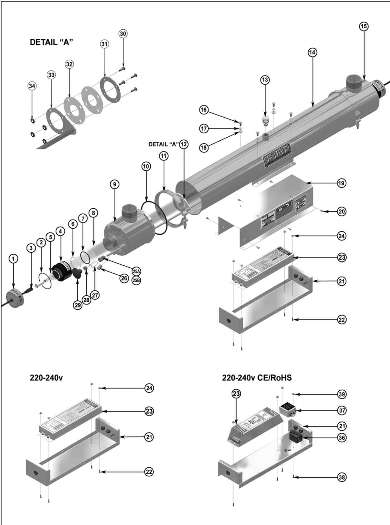
Figure 9 - Exploded View S2400C
