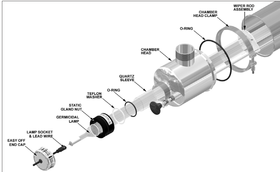
Figure 7 - Chamber Head Removal
