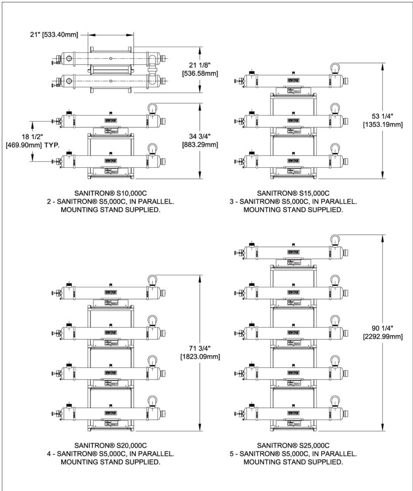
Figure 11 - S10,000C, S15,000C, S20,000C, S25,000C Dimensional Data
